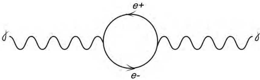
Figure 9-3. This 'Feynman diagram' is one expression of the non/emptiness of the void. It represents the void performing a vacuum fluctuation (just one of an infinite number of fluctuations of the void in its specific structuration). This one shows the virtual creation and annihilation of an electron-positron pair (which are jointly created and annihilated, and where the positron is an anti-electron, that is, its anti-matter partner). This can also be understood as a photon self-energy diagram. Wavy lines represent photons (quanta of the electromagnetic field, or light-particles, a particular case of which might be a gamma ray or high-energy radiation relevant to nuclear decay), while solid lines are electrons (and positrons): e^- represents a virtual electron traveling forward in time, and e^+ a virtual positron
